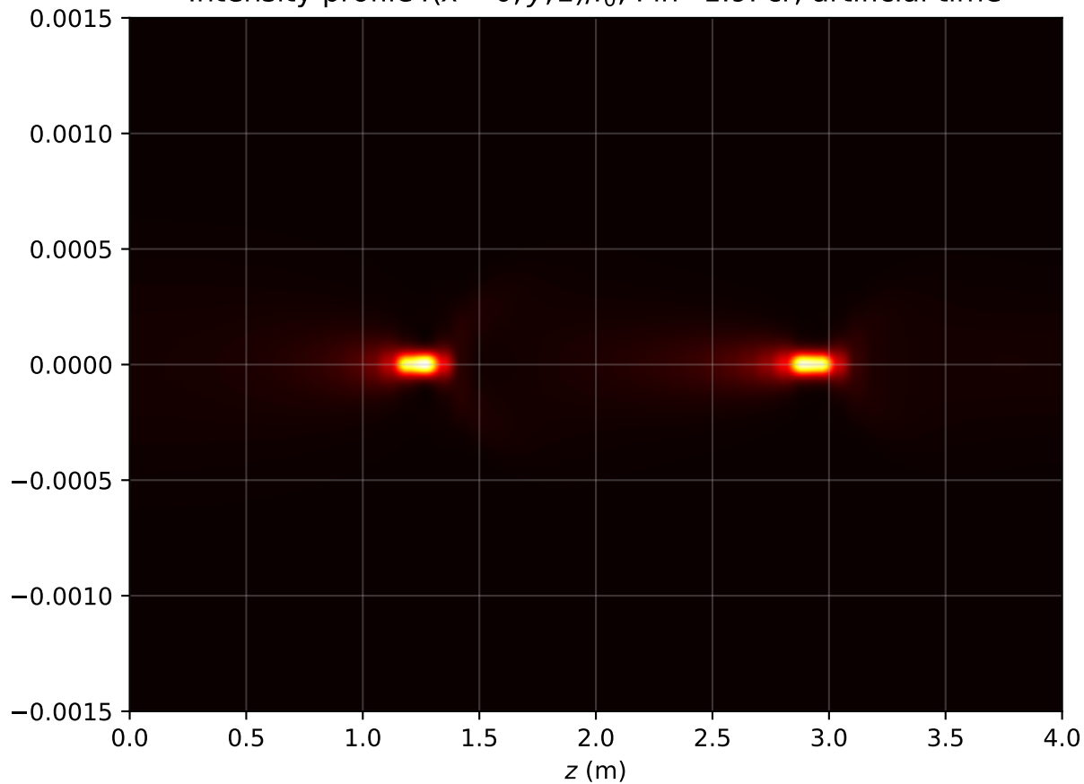
Intensity profile I(x=0, y, z)/I_0 , P_{in}=1.9P_{cr} , artificial time
